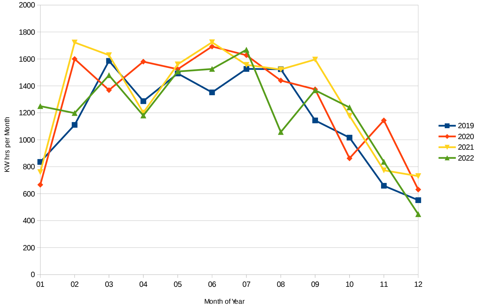
Solar Output Month/Year comparison
